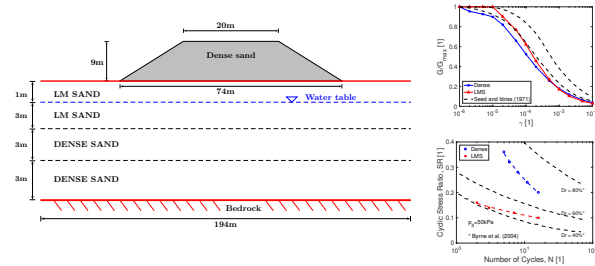
Figure 1: Geometry and behavior of the soils used for the numerical model (Lopez-Caballero and Khalil, 2018)
