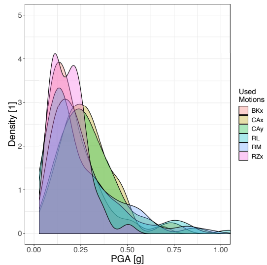
Figure 3: Density distribution function of the synthetic ground motions
