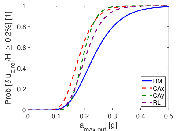
Figure 9: Fragility curves of the synthetic motions of Code Aster (CAx,CAy) and the real compatible motions
