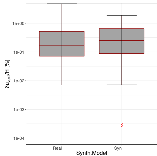
Figure 5: Box plot of the relative crest settlement for the tested motions
