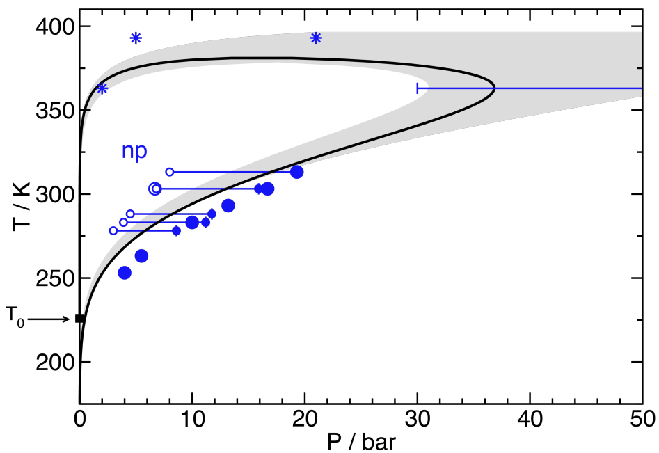
Figure 5: Temperature - CO 2 pressure phase diagram of amino-MIL-53(Al). Solid line: osmotic thermodynamic model. Grey zone corresponds to an arbitrary uncertainty of \pm 1 kJ.mol -1 introduced in the osmotic potential. Filled and open symbols are experimental transition steps in the adsorption and desorption isotherms respectively. The two distinct sizes of symbols correspond to two sets of experiments performed on different samples. The stars correspond to estimates of transition pressure for the two highest temperatures experimental adsorption isotherms measurements using the osmotic thermodynamic model. T_0 is the equilibrium phase transition temperature between the lp and np phases at zero pressure (i.e. the empty material).
