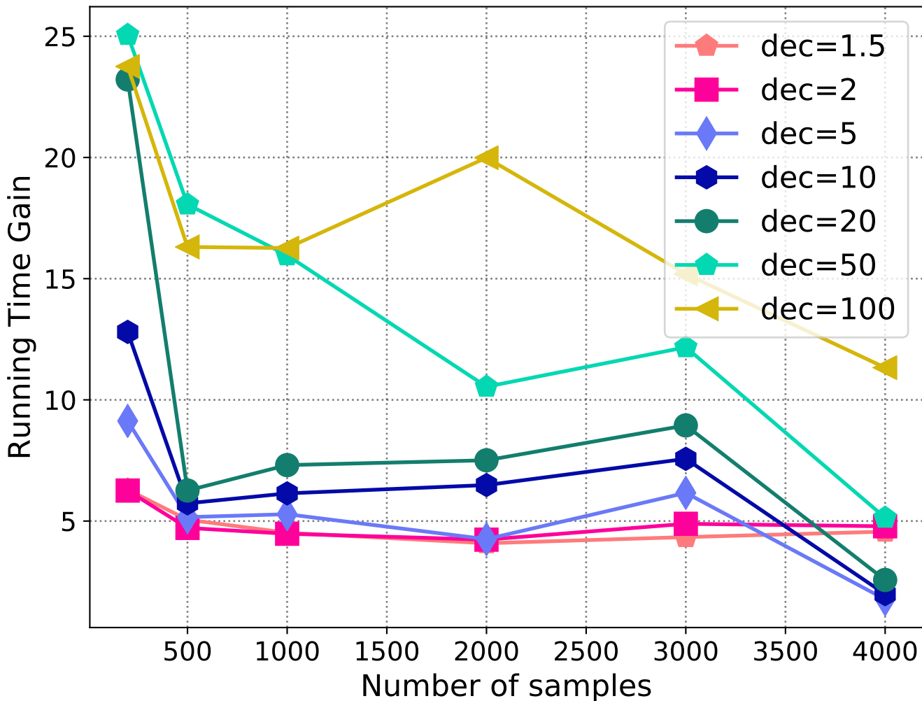
Screened WDA on mnist
