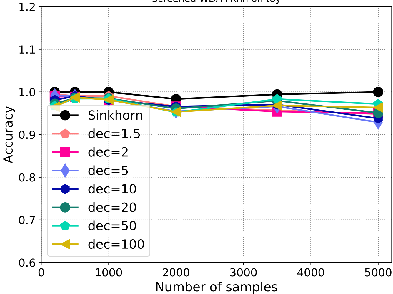
Screened WDA+Knn on toy
