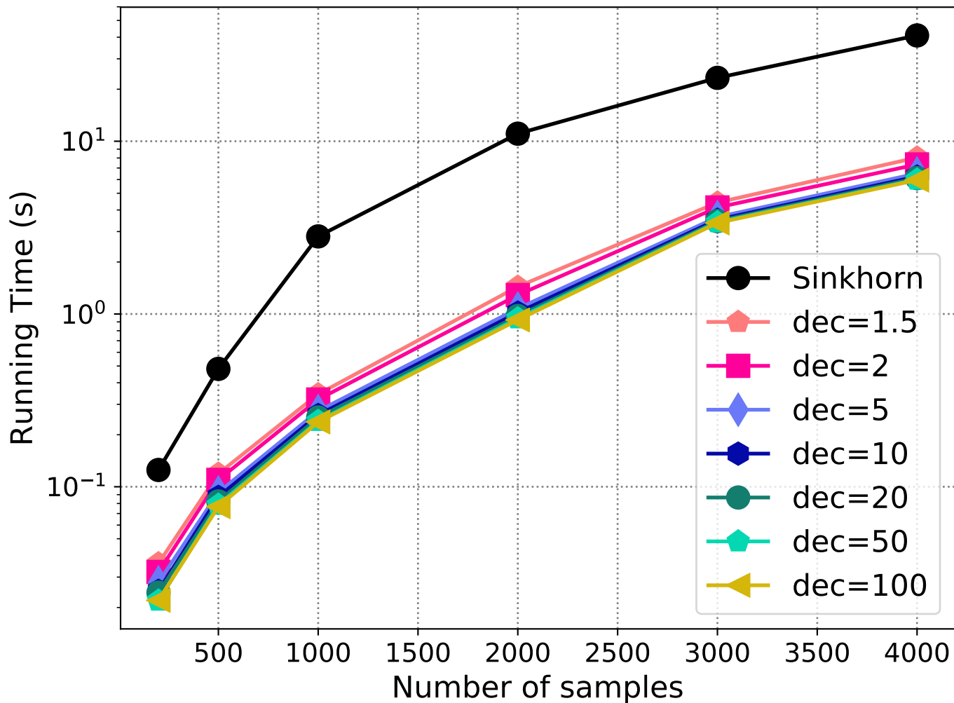
Screened OTDA on mnist
