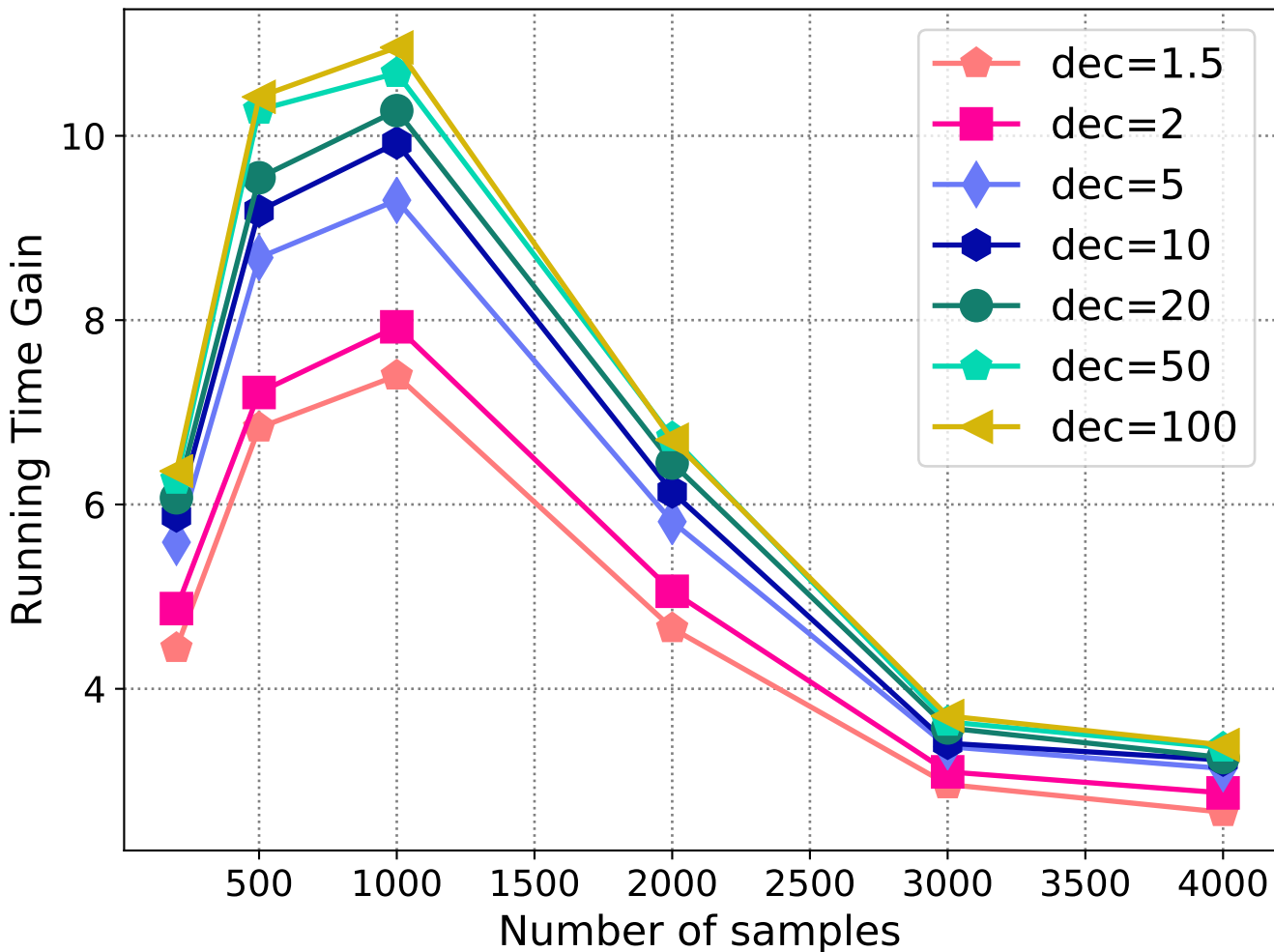
Screened OTDA on mnist
