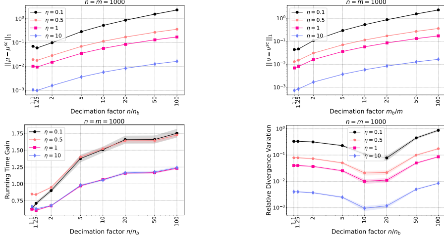
Figure 3: Empirical evaluation of Screenhorn vs Sinkhorn for normalized cost matrix i.e. \|C\|_\infty = 1 . Top panel: marginal violations in relation with the budget of points. Bottom panel: (left) ratio of computation times \frac{T_{\text{Sinkhorn}}}{T_{\text{Screenhorn}}} and, (right) relative divergence variation. The results are averaged over 30 trials.
