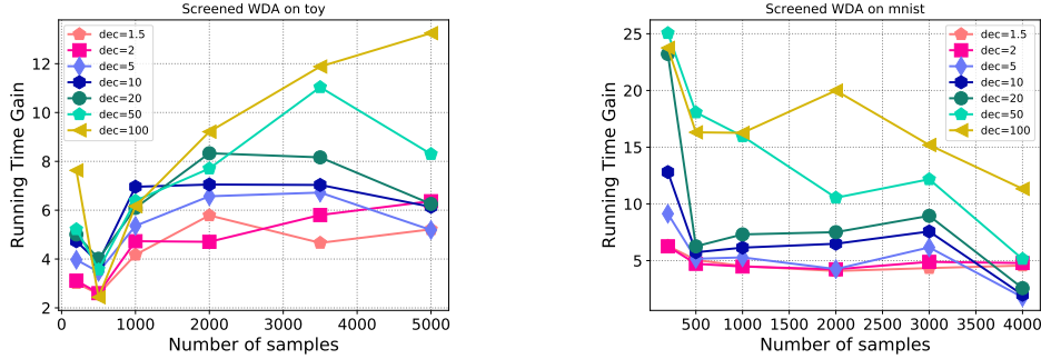
Figure 4: Wasserstein Discriminant Analysis : running time gain for a toy dataset and for MNIST as a function of the number of examples and the data decimation factor in Screenhorn .
