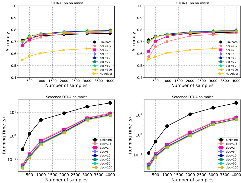
Figure 8: OT Domain adaptation MNIST to USPS : (top) Accuracy and (bottom) running time of Sinkhorn and Screenhorn for hyperparameter of the \ell_{p,1} regularizer (left) \lambda = 1 and (right) \lambda = 10 . Note that this value impacts the ground cost of each Sinkhorn problem involved in the iterative algorithm. The accuracy panels also report the performance of a 1-NN when no-adaptation is performed. We remark that the strength of the class-based regularization has influence on the performance of Screenhorn given a decimation factor. For small value on the left, Screenhorn slightly performs better than Sinkhorn, while for large value, some decimation factors leads to loss of performances. Regarding, running time, we can note that Sinkhorn is far less efficient than Screenhorn with an order of magnitude for intermediate number of samples.
