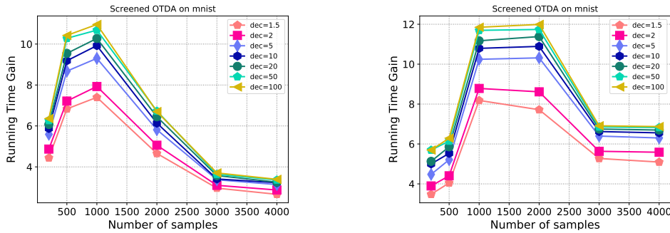
Figure 5: OT Domain adaptation : running time gain for MNIST as a function of the number of examples and the data decimation factor Screenhorn . Hyperparameter values (left) 1. (right) 10.
