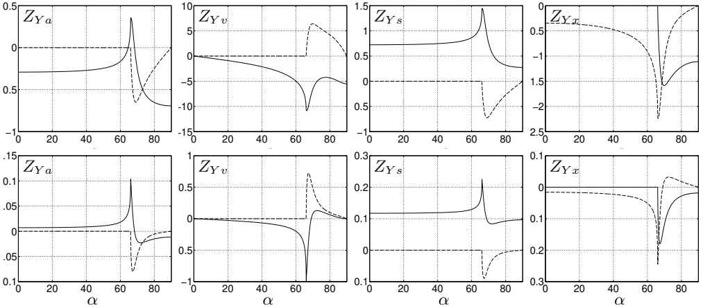
Figure 6: Real part (plain line) and imaginary part (dashed) of Z_{Yi} as a function of the incident wave angle \alpha , for different incident mass fraction wave: (A_t^r, A_t^c) = (1,0) (top), (0,1) (bottom). The remaining parameters are identical to Fig. 5: \gamma = 1.4 , M_1 = 2 and q = -2.25 . The corresponding emitted wave vector angle \alpha_s can be found in Fig 4.
