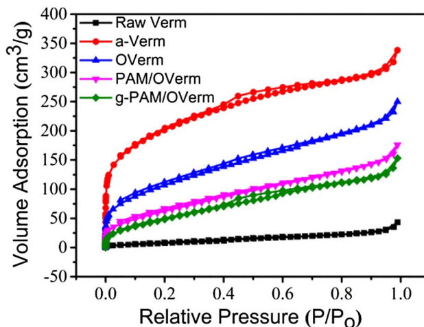
Fig. 14 \text{N}_2 adsorption-desorption isotherms of vermiculite (Raw Verm), acid-treated vermiculite (a-Verm), TEPM-modified vermiculite (OVerm), polyacrylamide/vermiculite (PAM/OVerm) and g -polyacrylamide/vermiculite ( g -PAM/OVerm), exhibiting type II isotherms with a hysteresis loop based on IUPAC classification, and the isotherm type for all vermiculite samples in the series is the same
