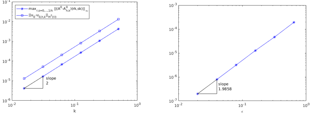
FIGURE 5. Approximation error for A^0 and u_0 for different values of k , using h = \frac{k}{4} , (left) and the squared error (4.8) in the approximation of u_\epsilon for different values of \epsilon (right).
