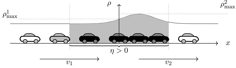
Figure 1: Illustration of the non-local traffic flow model (2.1) and (2.6) for different parameters on each road segment
