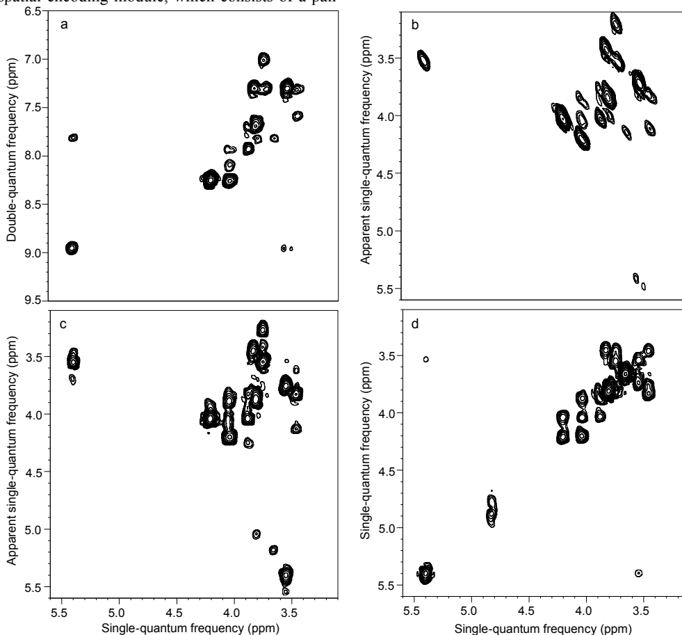
Fig. 2 Ultrafast NMR spectra of 0.1 M sucrose in D 2 O: a DQS (sequence shown in Fig. 1a); c DQSy (sequence shown in Fig. 1b); d COSY. All spectra were recorded in a single scan (2.2 s including water presaturation), using a double-quantum build-up delay \tau = 25 ms. Spectrum b was obtained from spectrum a by a shearing transformation at a processing stage. All spectra were recorded with a 600 MHz spectrometer equipped with a cryogenic probe.
