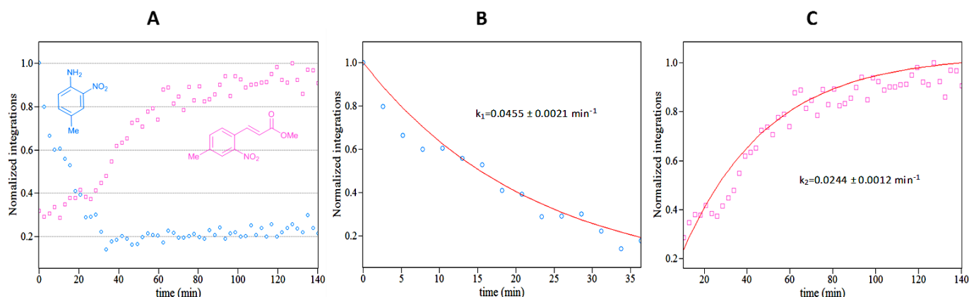
Fig. 3 Kinetics from the reaction monitoring ( A ) showing the evolution of normalized 2D peak volumes as the reaction progresses. These volumes were calculated from the cross-peaks (1) a,b and (3) b,a indicated in Figure 2, corresponding to the starting material and the final product, respectively. Blue open circles show the consumption of aniline and the pink open squares show the formation of the final styrene. The curves were obtained thanks to 55 UF COSY spectra recorded every 2.6 min. Kinetic constants can be extracted through exponential fitting of the 2D peak volumes in the relevant time domains, i.e. from 0 to 40 min for the consumption of aniline ( B ) and from 20 to 140 min for the production of the final styrene ( C )
