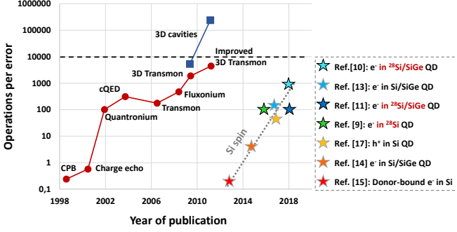
Fig. 2. Figure adapted from [16], showing the number of operations per error for various implementations of superconducting qubits vs. publication year. The added star symbols represent recent demonstrations of Si spin qubits. The figure of merit was estimated as the dephasing time T_2^* divided by the time needed to induce a \pi -rotation of the spin ( cf. angle \theta on the Bloch sphere Fig.1).
