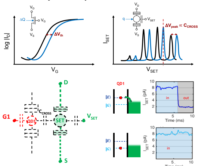
Fig. 8. Principle of single-shot detection through a coupled charge detector. (Top) In the same way that a charge coupled to the channel would shift the transfer characteristics of a MOSFET by \Delta V_{\text{th}} , a single charge event occurring near an SET causes a shift of the Coulomb peaks proportional to the cross-capacitance C_{\text{CROSS}} . (Bottom left) Charge detector coupled to a Quantum Dot. The spin-charge conversion mechanism is energy-selective readout [29], i.e. charge movement may occur for the excited spin state |E\rangle , but not for the ground state |G\rangle . Observing the current trace through the SET detector determines the spin state of the qubit in QD1.
