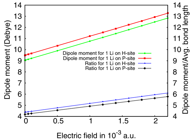
FIG. 2. Dipole moment and the ratio of dipole moment and average bond length between the alkali-metal atom and the carbon atom from the C_{60} vs electric field for one Li atom on the surface of a C_{60} .
