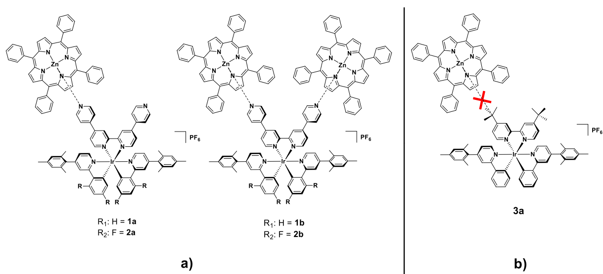
Chart 2. Chemical structures of a) the assemblies 1a [\text{Ir}(\text{mesppy})_2(\text{qpy})]\text{PF}_6 : \text{ZnTPP} 1:1 ratio and 2a [\text{Ir}(\text{dFmesppy})_2(\text{qpy})]\text{PF}_6 : \text{ZnTPP} 1:1 ratio; 1b [\text{Ir}(\text{mesppy})_2(\text{qpy})]\text{PF}_6 : \text{ZnTPP} 1:2 ratio and 2b [\text{Ir}(\text{dFmesppy})_2(\text{qpy})]\text{PF}_6 : \text{ZnTPP} 1:2 ratio, and b) Chemical structure of complex 3 mixed with ZnTPP ( 3a ) used as a control experiment.
