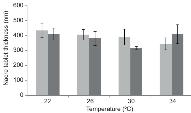
Fig. 4. Aragonite tablet thickness (nm) according to temperature and type of movement: random movement (light grey) and axial movement (dark grey) ( n=2-6 ). Data are means \pm s.d.
