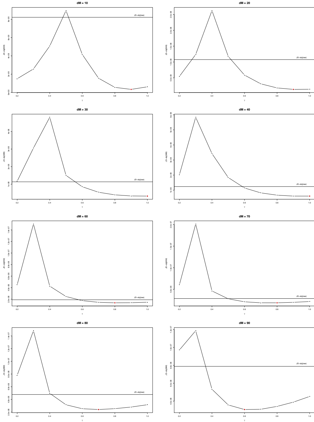
Figure 9: JD\text{-obj} values. JD\text{-obj}(MM) with different \gamma parameters and with d_M ranging from 10 to 90.
