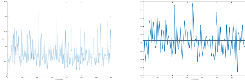
Figure 7: Unbiasedness . Estimates of \hat{\mathbf{c}}_{RR}^0 from different realizations. Left: 350 realizations; right: 140 realizations. We can find that the estimator is unbiased.
