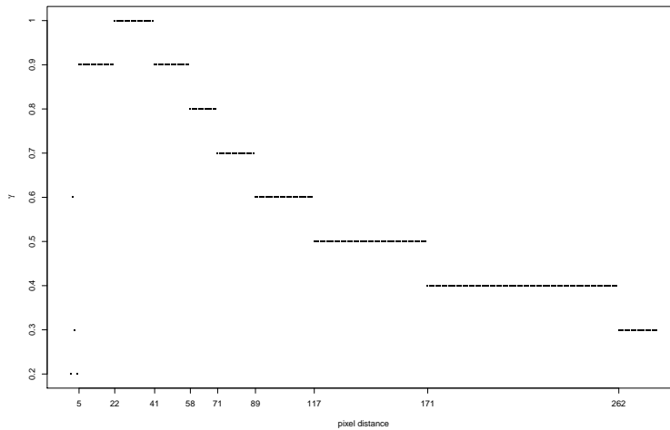
Figure 13: The best \gamma values for the families \{\hat{\mathbf{c}}^d\}_{d=0,\dots,d_M} . The x -axis records the moving of d_M .
