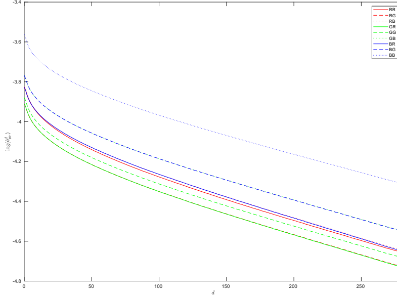
Figure 10: Exponential decay of covariance after the application of the Michaelis-Menten formula with \gamma = 0.7 . The choice of \gamma = 0.7 is arbitrary, but we stress that the exponential decay remains true also for all the other \gamma values that we have considered.
