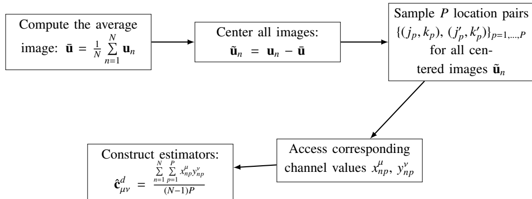
Figure 1: Construction of spatiochromatic covariance estimators.
