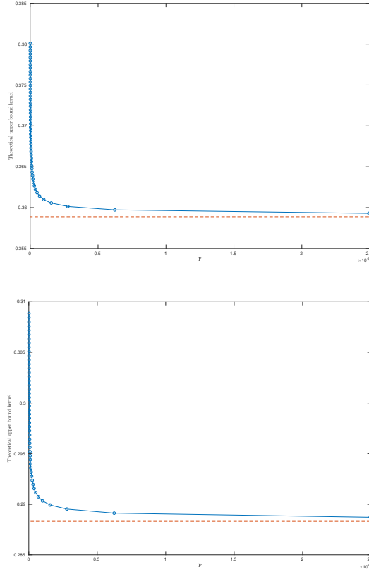
Figure 2: Theoretical upper bound kernel vs P. H = 1288 , W = 1936 , \beta = -0.0026 (top), -0.0020 (bottom). Right dashed line is the limit of the upper bound kernel.
