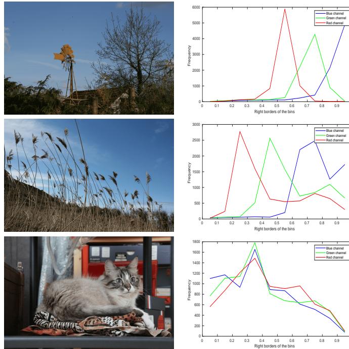
Figure 4: One typical distribution of sky images. The histogram is plotted with 10 bins and pixels are taken from the upper 1/3 part of the corresponding image.
