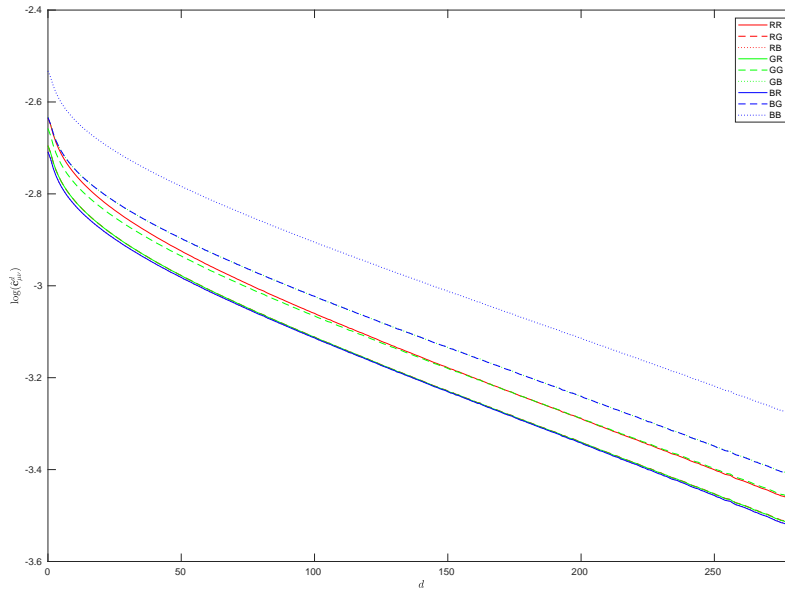
Figure 9: Exponential decay of raw images. We built the regression model and fit it with OLS on the range [70, 280] , where the covariances exhibit exponential decay precisely.
