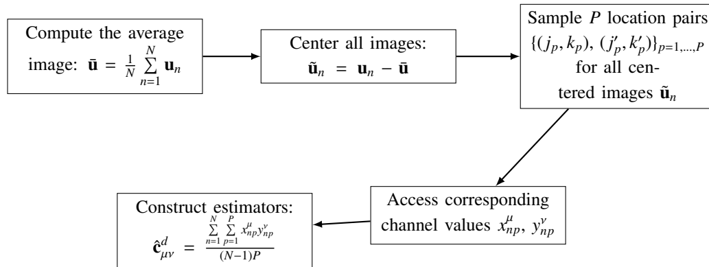
Figure 1: Construction of spatiochromatic covariance estimators.
