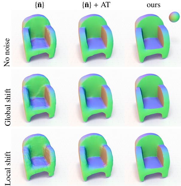
Figure 7: Robustness to misaligned normal maps. Here we simulate global misalignment by shifting an entire normal map by the same amount (second row) or by shifting each normal by a random amount (third row). While these perturbations degrades the result of the baseline methods, our method remains stable.
