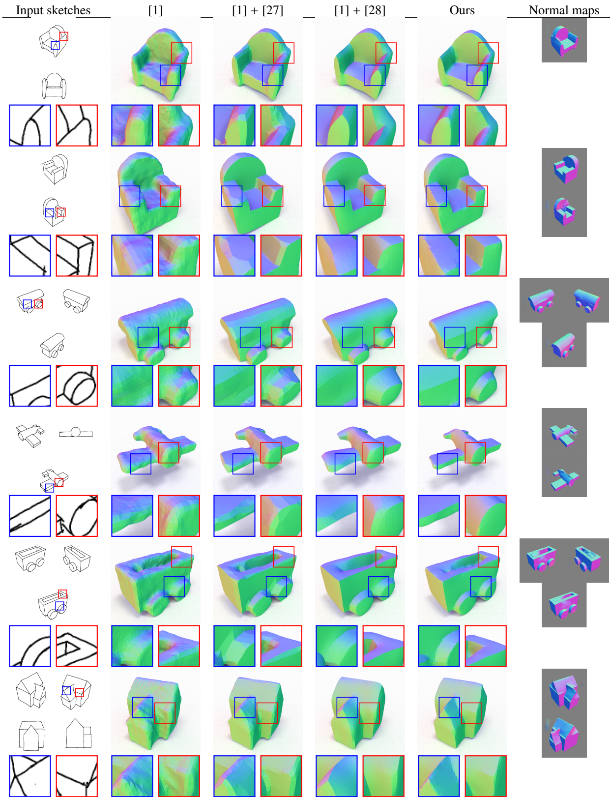
Figure 5: Comparison to Delanoj et al. [1] on a variety of objects. Applying marching cube on the volumetric prediction results in noisy surfaces that lack sharp discontinuities (second column). Denoising these surfaces with L_0 minimization [27] introduces spurious discontinuities as curved patches are approximated by planes (third column). Guided denoising [28] produces piecewise-smooth surfaces closer to ours (fourth column) but maintains low-frequency noise and tends to misplace discontinuities, like on the arm of the armchair (second row) or on the wings and front of the airplane (fourth row). Our formulation based on the Ambrosio-Tortorelli energy can be seen as a form of guided filtering that benefits from extra guidance from the predicted normal maps (fifth column). We included close-ups on the input drawings and output surfaces to show that our method better captures the intended shape.
