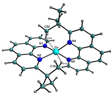
Fig. 5 Structure of the cation in (3)
