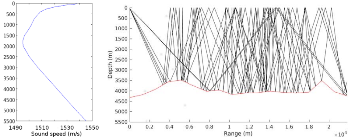
Fig.2: Sound speed profile-typical of Indian Ocean (left). OBS RR43: example of eigenrays tracing (right). Direct ray does not reach the OBS due to bottom profile, only reflected paths are possible.
