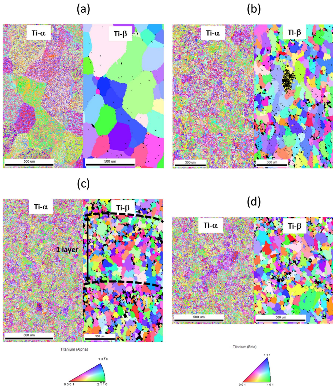
Fig. 10. EBSD analysis of Ti-6Al-4V α-Ti matrix and reconstruction of former β-grains for (a) 0% B 4 C, (b) 0.5% B 4 C, (c) 1.5% B 4 C, (d) 3% B 4 C (P400 V400) [17].
