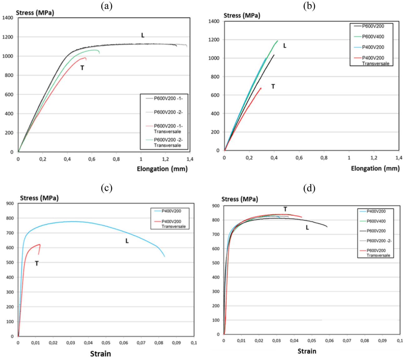
Fig. 15. Tensile tests on TMC for various process conditions: (a) Ti-6Al-4V at 20 °C, (b) Ti-6Al-4V + 1.5% B 4 C at 20 °C, (c) Ti-6Al-4V at 500 °C, (d) Ti-6Al-4V + 1.5% B 4 C at 500 °C.
