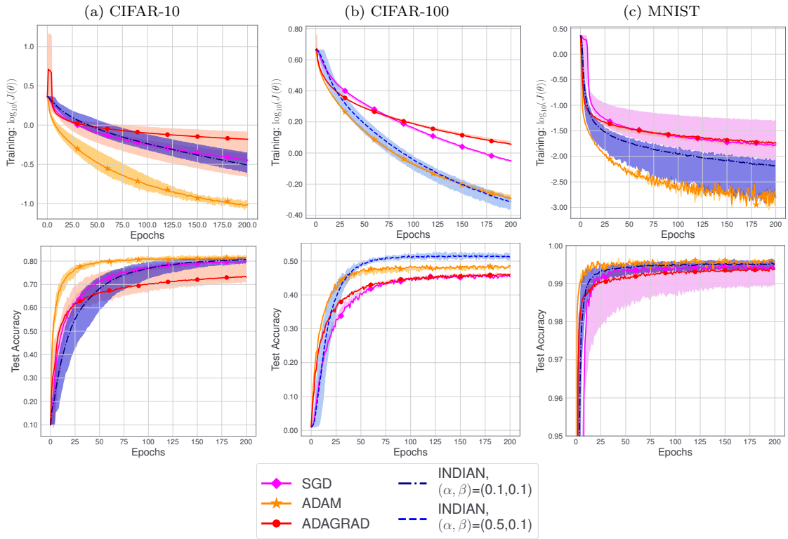
Figure 3: Comparison of INDIAN with state-of-the-art algorithms SGD, ADAM and ADAGRAD. Top: logarithm of the loss function \mathcal{J}(\theta) during the training. Bottom: classification accuracy on the test set.
