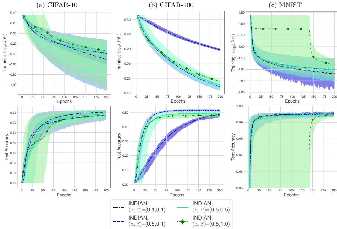
Figure 2: Analysis of the sensibility of INDIAN to the choice of \alpha and \beta using NiN for three different image classification problems. Top: logarithm of the loss function \mathcal{J}(\theta) during the training. Bottom: classification accuracy on the test set.
