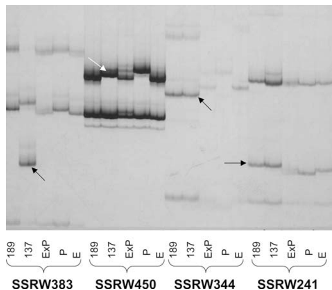
Fig. 1 Examples of markers showing new SSR alleles not present in the parents as revealed by silver-stained polyacrylamide gel electrophoresis in P lines 137 and 189. E × P Interspecific hybrid between the E and P parental species, arrows new bands
