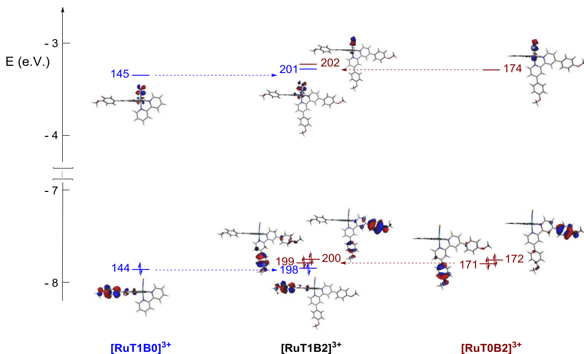
Figure 3 Main orbitals involved in the dominant low-energy transitions of [\text{RuT1B0}]^{3+} , [\text{RuT0B2}]^{3+} , and [\text{RuT1B2}]^{3+} .
