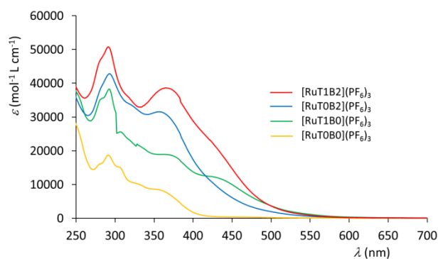
Figure 1 Comparison of the UV-visible spectra of the ruthenium complexes, in acetonitrile.
