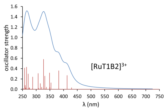
Figure 2 Comparison of the UV-visible spectra computed at the CAM-B3LYP/6-31G* level for the ruthenium nitrosyl complexes.
