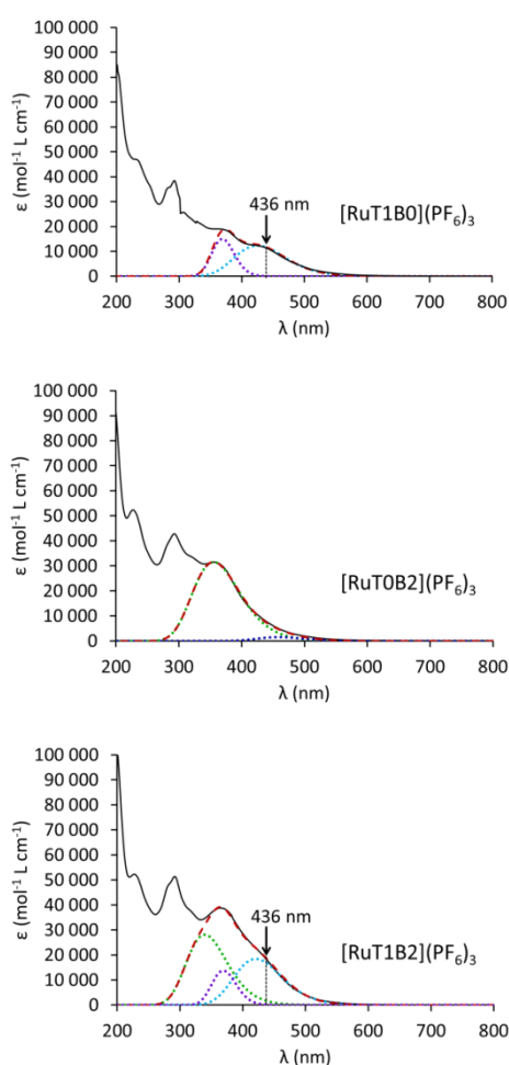
Figure 4 UV-visible spectra of [\text{RuT1B0}](\text{PF}_6)_3 , [\text{RuT0B2}](\text{PF}_6)_3 , and [\text{RuT1B2}](\text{PF}_6)_3 (black solid line) with deconvolutions: the red dashed lines are the sum of the contribution of dotted lines (see text).
