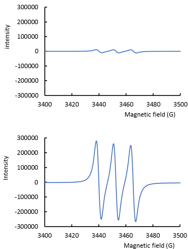
Figure 6 Representative triplet signal from NO • trapped by [Fe II (MGD) 2 ] in acetonitrile, after irradiation of [RuT0B2](PF 6 ) 3 , with a Hg lamp (bottom). The signal recorded before irradiation is given as a reference (top).
