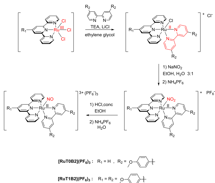
Scheme 2 Synthetic route towards [RuT0B2](PF 6 ) 3 and [RuT1B2](PF 6 ) 3 .
