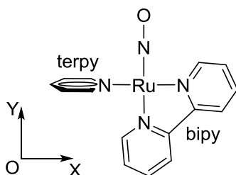
Scheme 3 Partial coordination sphere in the XY plane for a [\text{Ru}(\text{terpy})(\text{bipy})(\text{NO})]^{3+} species in the case of an ideal \text{RuN}_6 octahedral symmetry.
