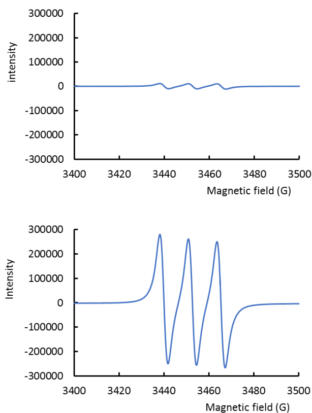
Figure 6 Representative triplet signal from \text{NO}^\cdot trapped by [\text{Fe}^{\text{II}}(\text{MGD})_2] in acetonitrile, after irradiation of [\text{RuT0B2}](\text{PF}_6)_3 , with a Hg lamp (bottom). The signal recorded before irradiation is given as a reference (top).
