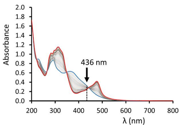
Figure 5 Changes in the absorption spectrum of [\text{RuT1B2}](\text{PF}_6)_3 , in acetonitrile, under irradiation at \lambda = 436 nm. The blue curve corresponds to the starting complex and the red curve corresponds to the photo-product.
