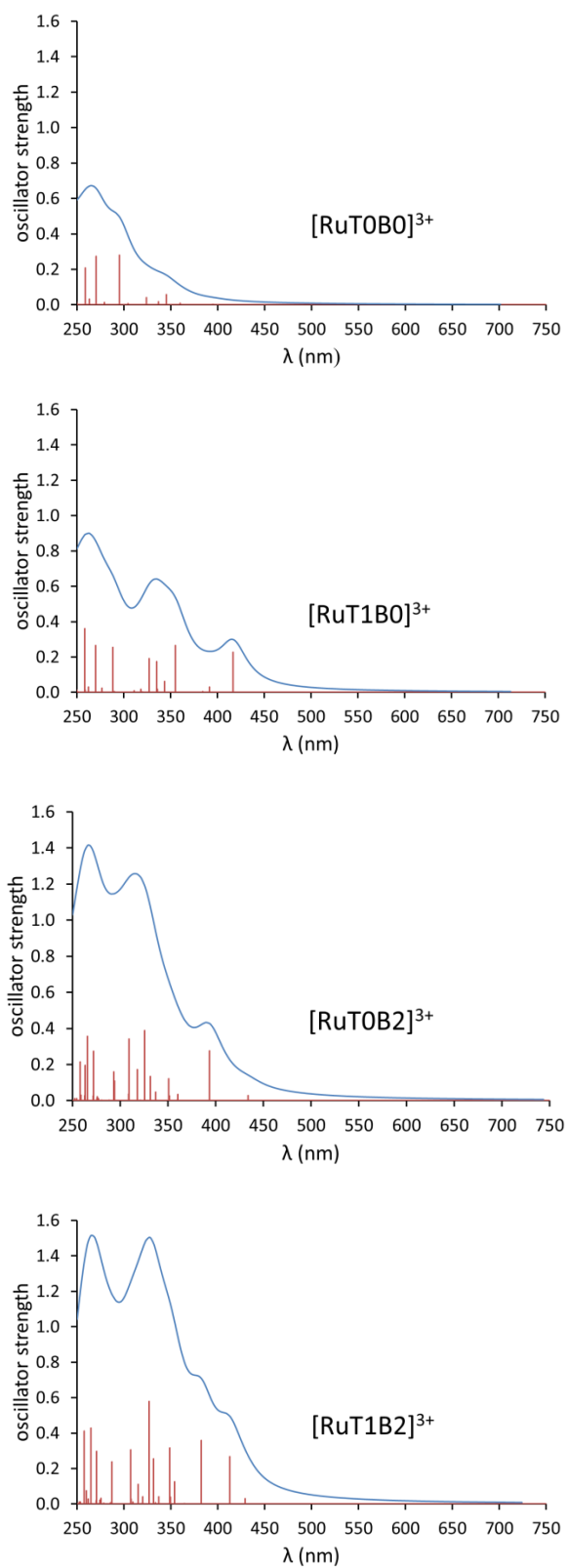
Figure 2 Comparison of the UV-visible spectra computed at the CAM-B3LYP/6-31G* level for the ruthenium nitrosyl complexes.
