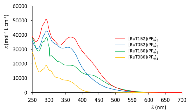
Figure 1 Comparison of the UV-visible spectra of the ruthenium complexes, in acetonitrile.
