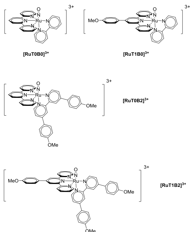
Scheme 1 [Ru(terpy)(bipy)(NO)] 2+ complexes with 0, 1, 2, and 3 methoxyphenyl substituents.
