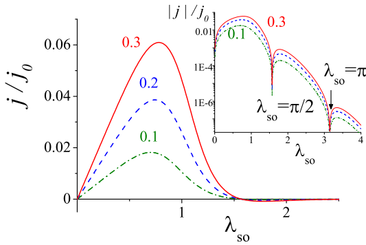
FIG. 4. The dependence of the current density j on spin-orbital constant \lambda_{SO} for different temperatures T < T_c [ j_0 = 4e(\hbar/R)^3\gamma^2/b ]. The numbers by the curves correspond to the dimensionless shift \Delta\tau = (R/\xi_0)^2(T_c - T)/T_c in T with respect to the transition (4).
