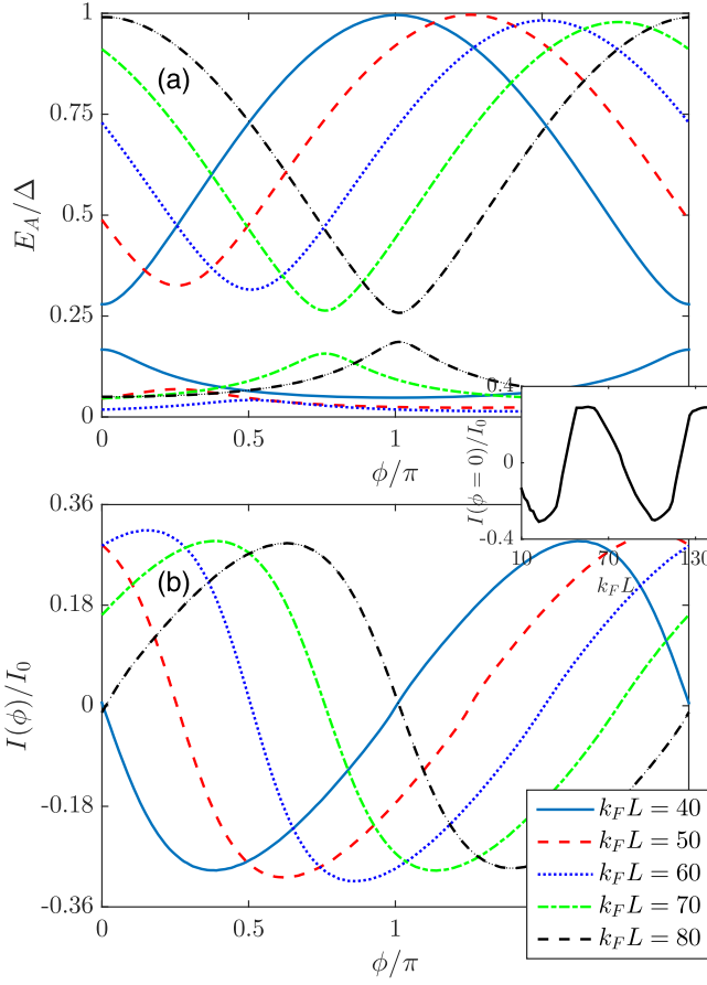
FIG. 9. (a) Andreev bound-state energies vs the superconducting phase difference \phi and (b) current-phase relation for a conical half-metallic junction when k_F L varies from 40 to 80 with steps of 10. The inset shows the dependence of I(\phi = 0) on the thickness k_F L . Here we set the parameters E_F = 1000\Delta , h/E_F = 0.55 , h_z/E_F = 0.084 , and Q/k_F = \pi/2 .
