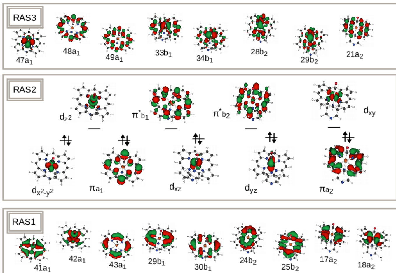
Figure 2: Active orbitals obtained after an eight roots state averaged RASSCF-28e26a calculation of A_1 symmetry for the FeP(pz)CO complex.
