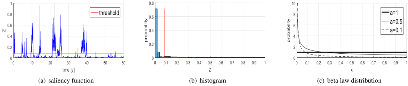
FIGURE 2 – Resulting saliency function (a) and its histogram (b) computed from the recursive synchrosqueezed STFT of an EEG signal. Its probability density function can be compared to a beta distribution (c) with parameter a \in \{0.1, 0.5, 1\} .
