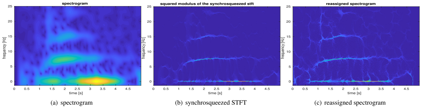
FIGURE 1 – Comparisons of the different recursive TFRs computed for an EEG signal with a HVS.
