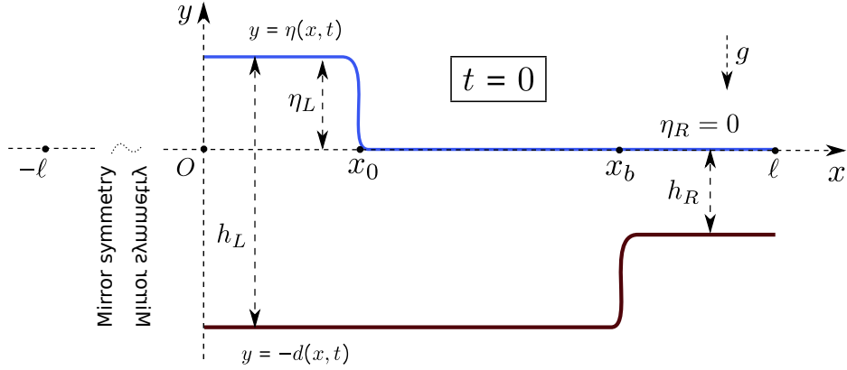
Figure 2. Sketch of the numerical test case considered in section 3.
