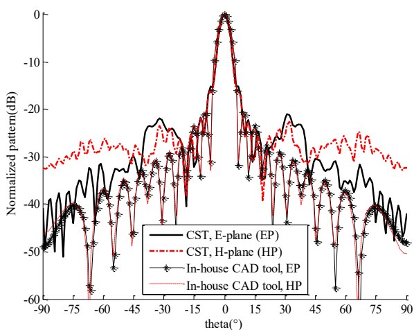
Fig. 5. Computed normalized co-polarization radiation patterns of MOTA#1 at 29.5 GHz in E- and H-planes (EP and HP).
