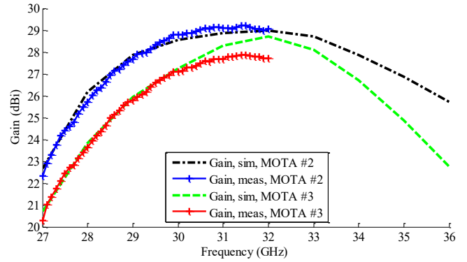
Fig. 8. Simulated and measured co-polarized gains of MOTA#2 and MOTA#3 at up-link Ka-band.
