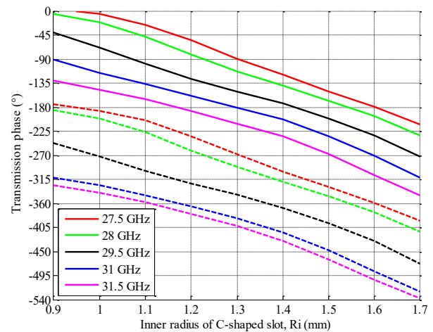
Fig. 3. Transmission phase of the MOUC with respect to the inner radius R_i of the C-shaped slot for various frequencies. Solid lines refer to clock-wise model (Fig. 1a) and dashed lines refer to counter-clockwise model (Fig. 1b).
