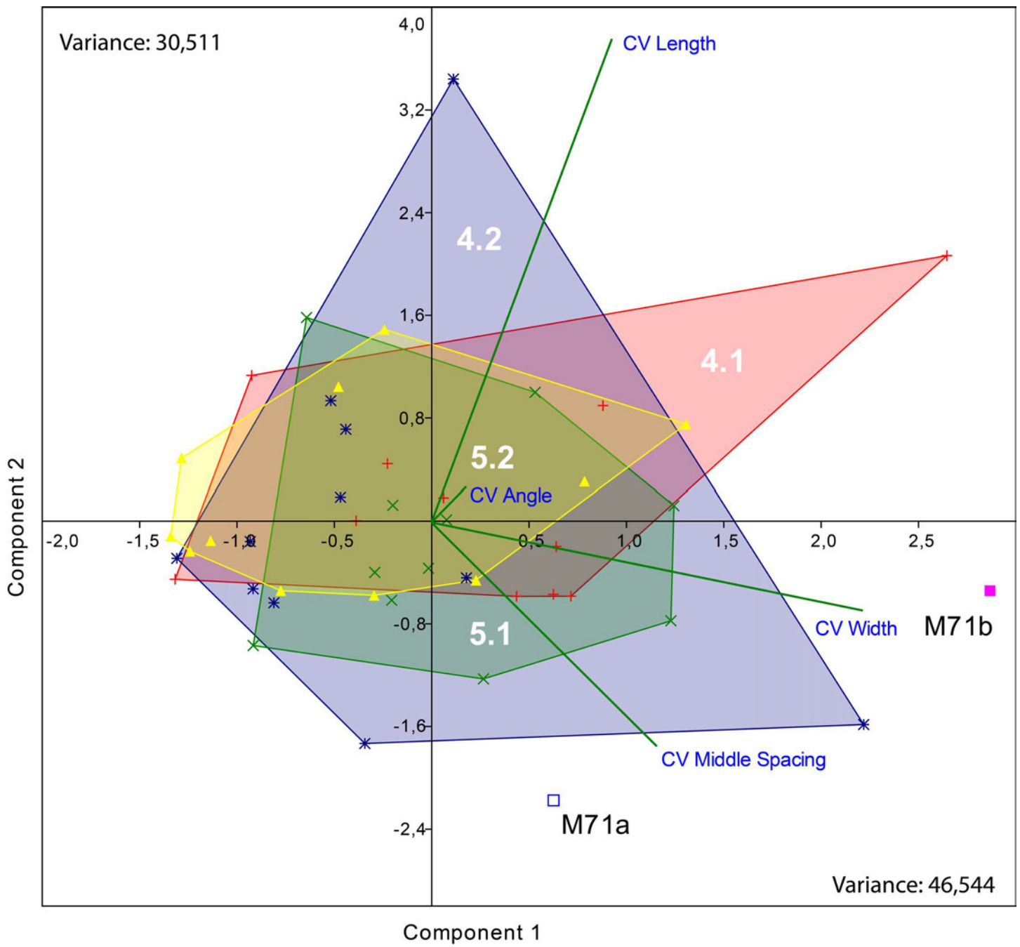
SM Figure 16. PCA scatter diagram of subsets of incisions produced by modern subjects during phase 4 and 5 of the experiment and subsets a and b incised on Les Pradelles M71 specimen.
