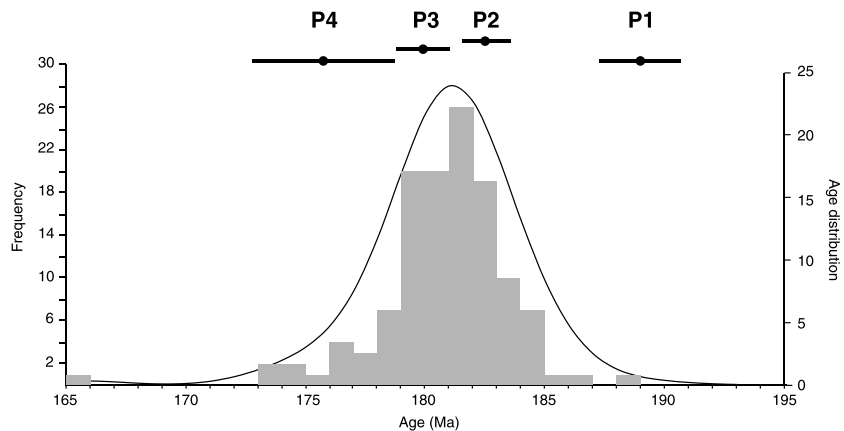
Figure 14. ^{40}\text{Ar}/^{39}\text{Ar} age probability density distribution diagram and frequency histogram of 125 rocks of the Karoo-Ferrar province [Heimann et al. , 1994; Duncan et al. , 1997; Fleming et al. , 1997; Minor and Mukasa, 1997; Elliot et al. , 1999; Jones et al. , 2001; Le Gall et al. , 2002; Jourdan et al. , 2004, 2005, 2007a, 2007b, 2008; Riley et al. , 2006; and this study]. Volcanic phases P1 to P4 described in the text are roughly indicated.
