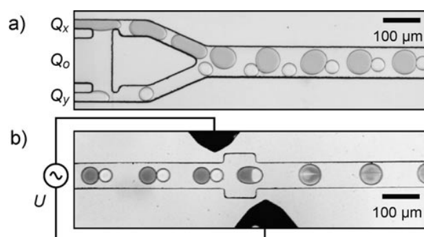
Figure 17: a) Pairing module. Two aqueous phases are injected by the outer channels and are synchronously emulsified by the central oil channel. The flow rates are Q_o=800 \text{ mLh}^{-1} for the oil and Q_x=400 \text{ mLh}^{-1} , Q_y=100 \text{ mLh}^{-1} for the aqueous phases. b) Fusion module. Paired droplets can be coalesced by applying an electrical voltage U between the two electrodes. Q_1=650 \text{ mLh}^{-1} , Q_2=100 \text{ mLh}^{-1} , Q_3=60 \text{ mLh}^{-1} . Reprinted with permission from ref[96]. Copyright 2008 Wiley.
