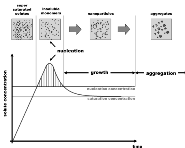
Figure 4: Cartoon illustration of nucleation and growth during the preparation of monodisperse nanoparticles. Reprinted with permission from ref[23]. Copyright 2004 Royal Society of Chemistry.
