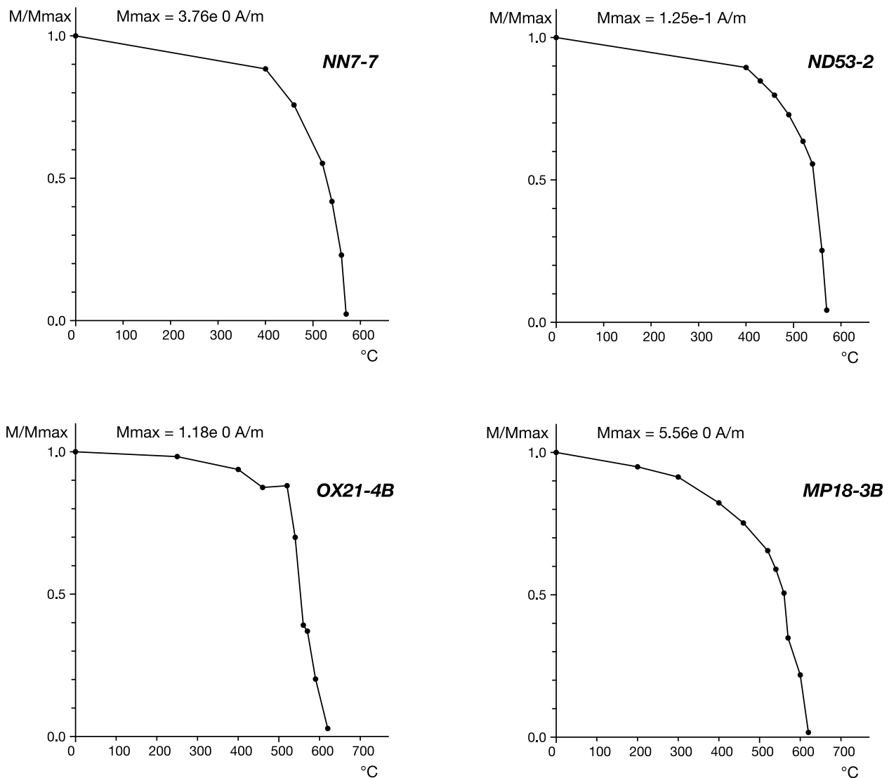
Figure 6. Four representative thermal demagnetization diagrams of samples from the Naude's Nek (NN, ND) and Oxbow-Moteng Pass (OX, MP) sections selected for measurement of relative paleointensity as explained in the text.
