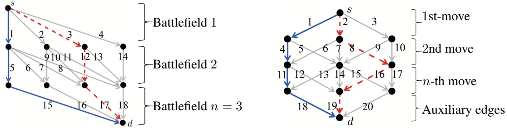
(a) The graph G_{3,3} corresponding to the CB game with k = n = 3 . E.g., the bold-blue path represents the strategy (0, 0, 3) while the dash-red path represents the strategy (2, 0, 1) . (b) The graph G_{3,3,1} corresponding to the HS game with k = n = 3 and \kappa = 1 . E.g., the blue-bold path represents the (1, 1, 1) search and the red-dashed path represents the (2, 3, 2) search.
