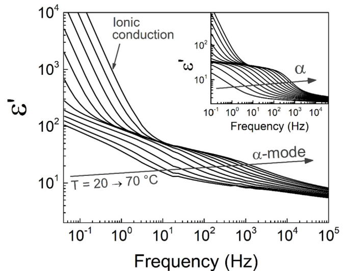
Fig. 3. Isothermal relative permittivity spectra (real part of \epsilon^* ) obtained from the EIS measurements on the epoxy varnish (2 weeks of immersion in 0.5 M NaCl). Inset: BDS spectra of the dry epoxy varnish, in the temperature range [50; 100 °C]. For the sake of readability, the 8 experimental points per decade are represented as continuous lines.
