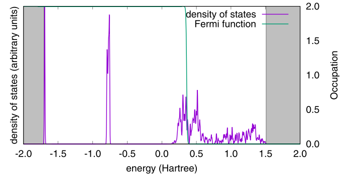
Fig. 2. Density of states for the 9 \times 9 \times 9 supercell (containing 1458 atoms) of bcc Niobium. Compared to Fig. 1, the spectral width is larger due to the inclusion of semicore electrons.
