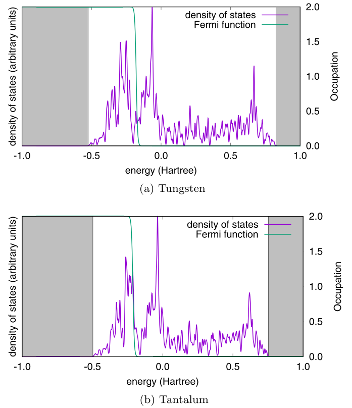
Fig. 1. Density of states for the 9 \times 9 \times 9 supercell (containing 1458 atoms) of bcc Tungsten and Tantalum. The spectral width is very small, which is a direct consequence of the usage of pseudopotentials and of the special properties of the support functions used by BIGDFT.
