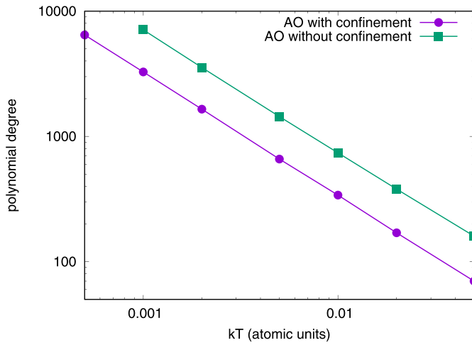
Fig. 3. Polynomial degree used by the FOE method within CHES as a function of the electronic temperature, for two set of atomic orbitals (AO). The set that was obtained by solving the atomic Schrödinger equation with a confining potential leads to considerably lower values due to its smaller spectral width.
