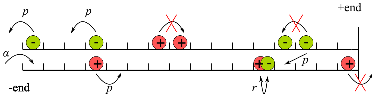
Figure 1. Schematic drawing of the possible transitions in the two lane model. Red (plus) particles hop with rate p from left to right. Green (minus) particles hop with rate p from right to left. Minus particles change lane with rate p if the next site on their lane is occupied while it is empty on the other lane. Particles transmute with rate r . Injection of plus particles occurs with rate \alpha on both entrance sites on the left, if they are empty. Minus particles located on the leftmost sites leave the system with rate p .
