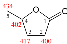
Figure 4: \gamma -valerolactone with atom labels (black) and C-H bond dissociation energies (red) in kJ/mol [8].
