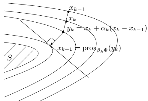
Inertial Proximal algorithm.
