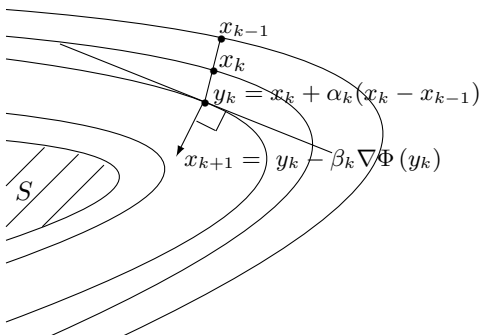
FIGURE 1. Inertial Gradient algorithm
