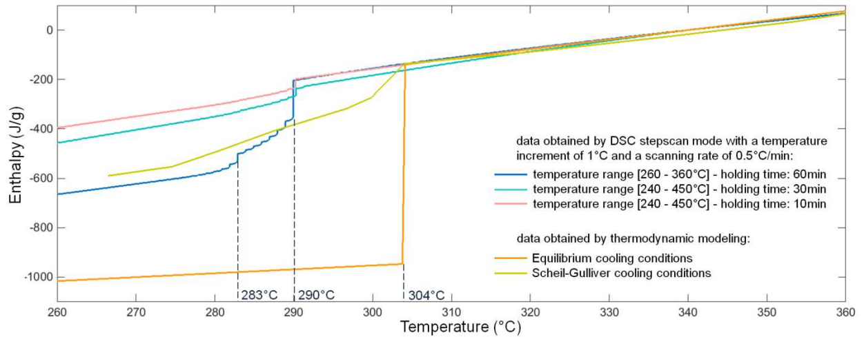
Figure 8. Experimental enthalpy evolutions of \text{Li}_4\text{Br}(\text{OH})_3 (with respect of the enthalpy of reference) with temperature, at ambient pressure, obtained with three different protocols by DSC stepscan mode and compared with the calculated ones, at equilibrium and Scheil-Gulliver cooling conditions.
