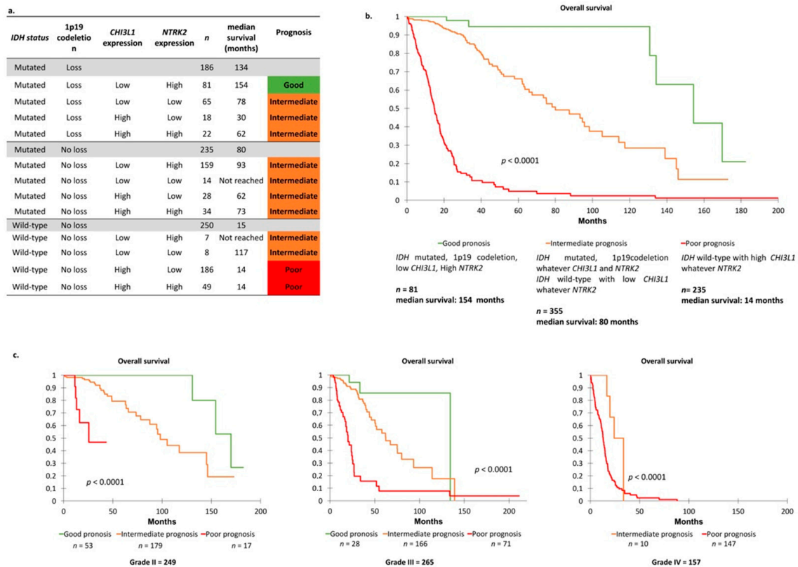
Figure 5. (a) Overall survival in glioma molecular groups according IDH status, 1p19 co-deletion and CHI3L1 and NTRK2 expression. (b) Overall survival in three glioma molecular groups by Kaplan–Meier analysis: Three groups with different prognoses were identified ( p < 0.0001 ). Three molecular groups were identified: Poor prognosis group combining IDH wild-type status, no co-deletion of 1p19q, high CHI3L1 expression and low NTRK2 expression; very good prognosis group combining IDH mutated, 1p19q co-deletion, low CHI3L1 expression and high NTRK2 expression; and intermediate prognosis group combining the other associations ( p < 0.0001 ). p -values were calculated using log-rank test. (c) Overall survival in each grade of glioma according to molecular group by Kaplan–Meier analysis: Three groups with different prognoses were identified ( p < 0.0001 ).
