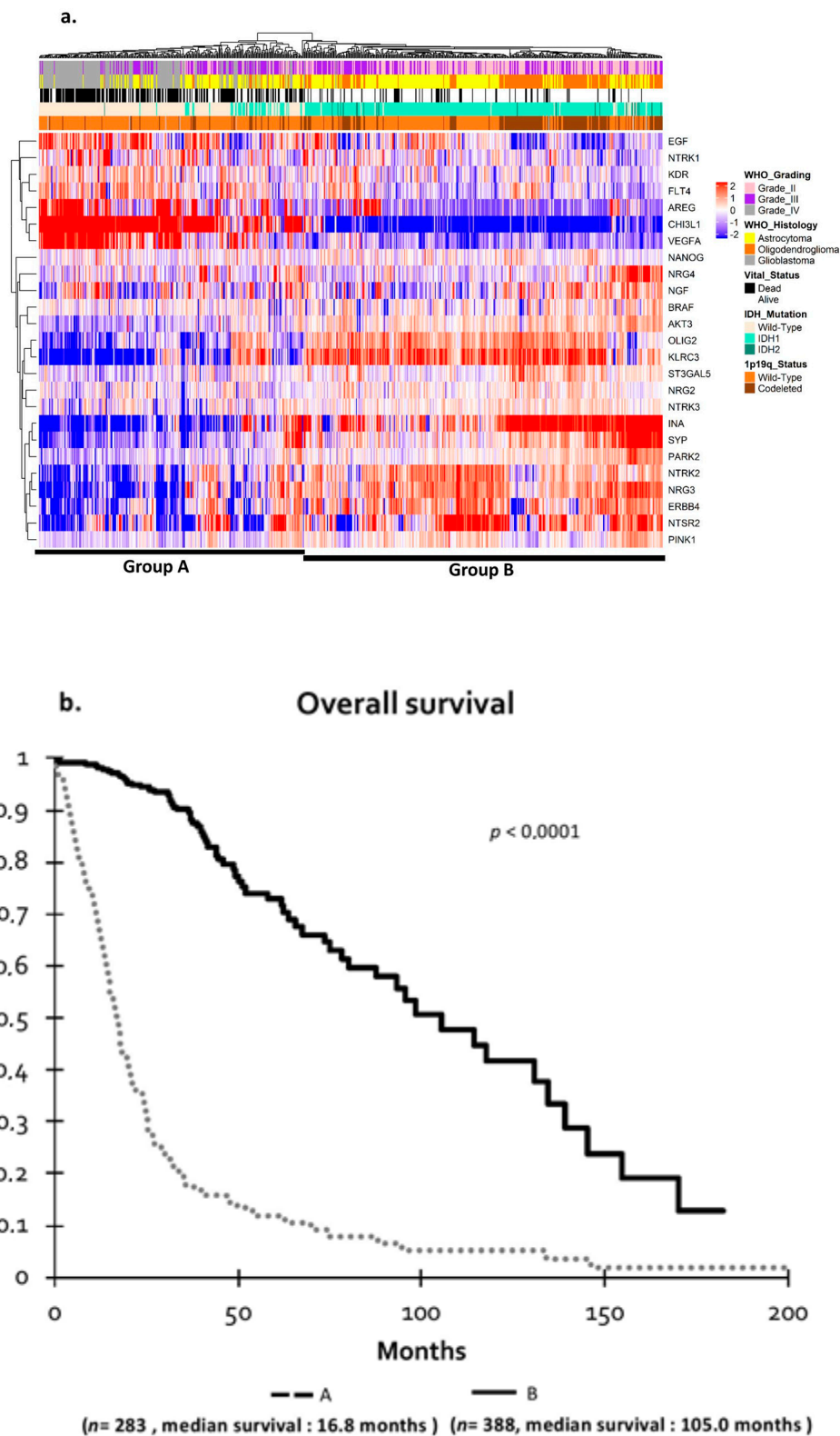
Figure 2. (a) Hierarchical clustering of brain tumors based on The Cancer Genome Atlas (TCGA) cohort: Hierarchical clustering of 671 gliomas based on 26 genes. Analysis of TCGA samples was performed as in Figure 1a. (b) Overall survival in TCGA cohort by Kaplan–Meier analysis. Survival group A (dotted line) defined unfavorable prognosis, and survival group B (bold line) defined favorable prognosis ( p = 0.007 ). p -values were calculated using log-rank test.
