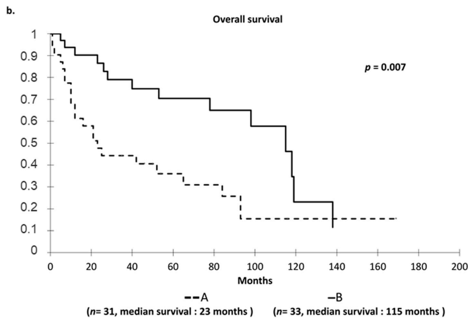
Figure 1. (a) Hierarchical clustering of brain tumors based on expression profiles of 26 genes in studied cohort: log 2 -transformed and mean-centered fold-change values from 26 genes fulfilling the criterion of statistically significant deregulation between two stages of glioma ( p < 0.05 ). Red and blue indicate transcript levels above and below median values, respectively. Tumor samples are identified by numbers, and genes by their symbols. Each column indicates the gene expression profile of a sample, and each line indicates variations in the expression level of a given gene among tumor samples. The length of branches on trees forming dendrograms on top of each panel reflects the degree of similarity between samples. Subdivision of samples into two groups according to the dendrogram was subsequently used for survival analysis. (b) Overall survival in the studied cohort by Kaplan–Meier analysis: Survival group A (dotted line) defined unfavorable prognosis, and survival group B (solid line) defined favorable prognosis ( p = 0.007 ). P-values were calculated using log-rank test. Group A was defined by high expression of EGF , NGF , FLT4 , KDR , AREG , NTRK1 , VEFGA and CHI3L1 and low expression of SYP , INA , ST3GAL5 , OLIG2 , KLRC3 , NTSR2 , PINK1 , NRG3 , ERBB4 , NTRK2-FL , NTRK2-T1 , AKT3 , PARK2 , NANOG , NTRK3 , NRG2 , BRAF and NRG4 , whereas group B was defined by the opposite pattern of gene expression.
