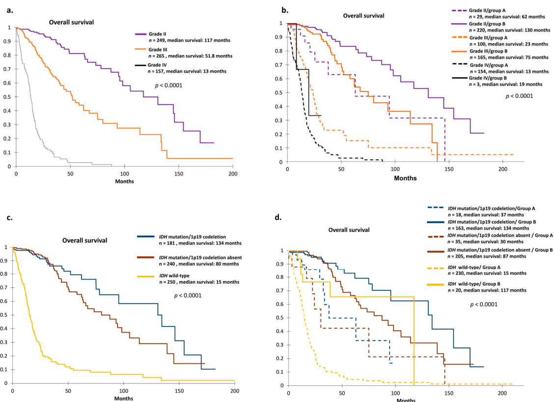
Figure 3. (a) Overall survival curves according to grade in TCGA cohort by Kaplan–Meier analysis. p -values were calculated using log-rank test. (b) Overall survival curves according to grade and 26-gene signature in TCGA cohort. Survival group A (dotted line) defined unfavorable prognosis, and survival group B (solid line) defined favorable prognosis ( p < 0.0001 ) by Kaplan–Meier analysis. In subgroups for each grade, the 26-gene signature provided information about prognosis. p -values were calculated using log-rank test. (c) Kaplan–Meier overall survival curves according to molecular characteristics in TCGA cohort. p -values were calculated using log-rank test. (d) Overall survival curves according to molecular characteristics and 26-gene signature in TCGA cohort. Survival group A (dotted line) defined unfavorable prognosis, and survival group B (solid line) defined favorable prognosis ( p < 0.0001 ). In each subgroup of molecular characteristics, the 26-gene signature further refined prognosis. p -values were calculated using log-rank test.
