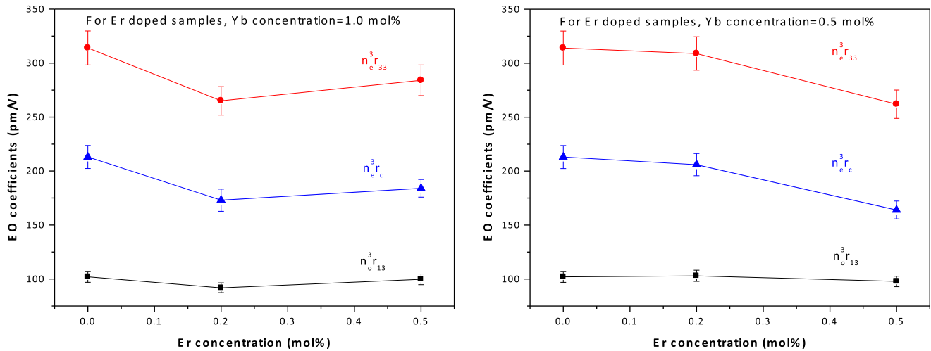
Fig. 2. The experimental n_o^3 r_{13} and n_e^3 r_{33} and calculated n_e^3 r_c figures of merit of lithium niobate crystals co-doped with \text{Er}^{3+} - \text{Yb}^{3+} as function of the concentration of dopant.
