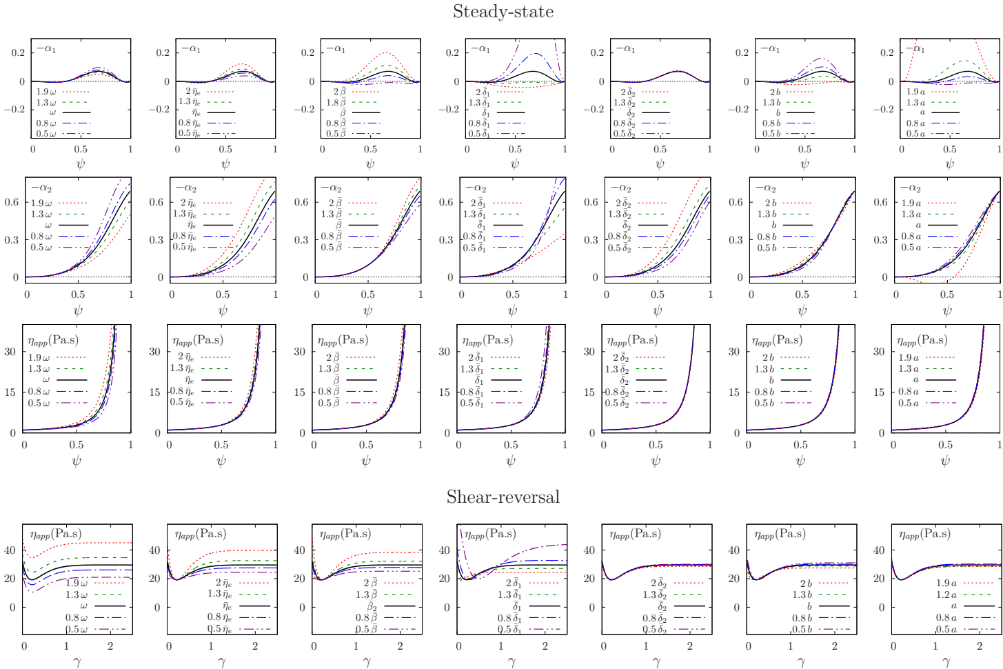
FIGURE 5. Upper three plot lines: Evolution of steady-state normal stress ratios \alpha_1 , \alpha_2 and apparent viscosity \eta_{app} versus reduced volume fraction \psi as the seven model constants \omega , \eta_e , \delta_1 , \delta_2 , a , b , \beta vary around their reference values indicated in table 1 (see legends). Lower plot line: Idem for the transient evolution of apparent viscosity \eta_{app} after a shear-reversal (case \phi = 0.44 and \phi_m = 0.535 ).
