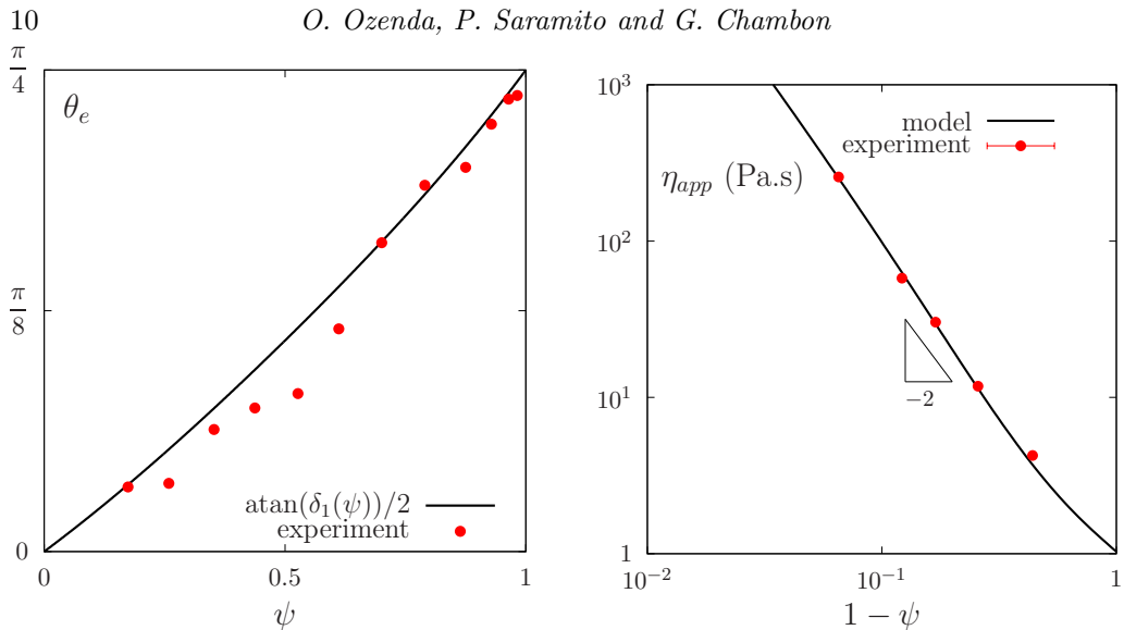
FIGURE 1. Evolution of depletion angle \theta_e and steady-state apparent viscosity \eta_{app} versus reduced volume fraction \psi : comparison between model predictions and experimental data of Blanc et al. (2013) ( \theta_e ) and Blanc et al. (2011) ( \eta_{app} ).
