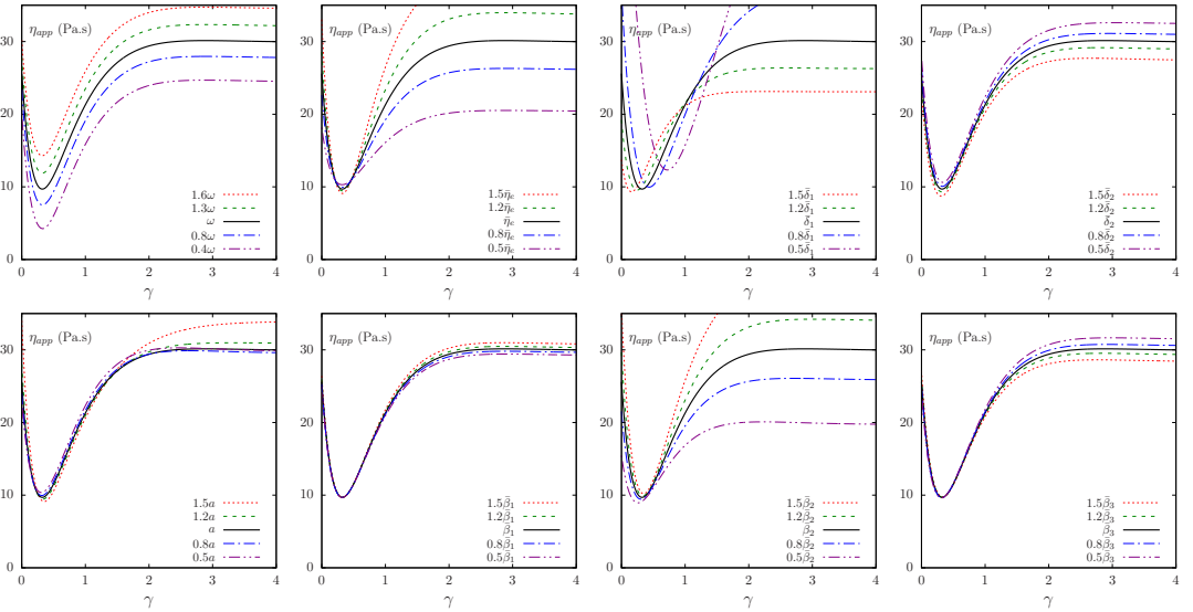
FIGURE 8. Sensitivity of transient apparent viscosity \eta_{app} with respect to model constants. Each of the constants was varied around the reference values indicated in table 1.
