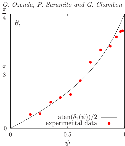
FIGURE 1. Depletion angle \theta_e versus reduced volume fraction \psi : comparison between model prediction (3.5a) and experimental measurements of Blanc et al. (2013).
